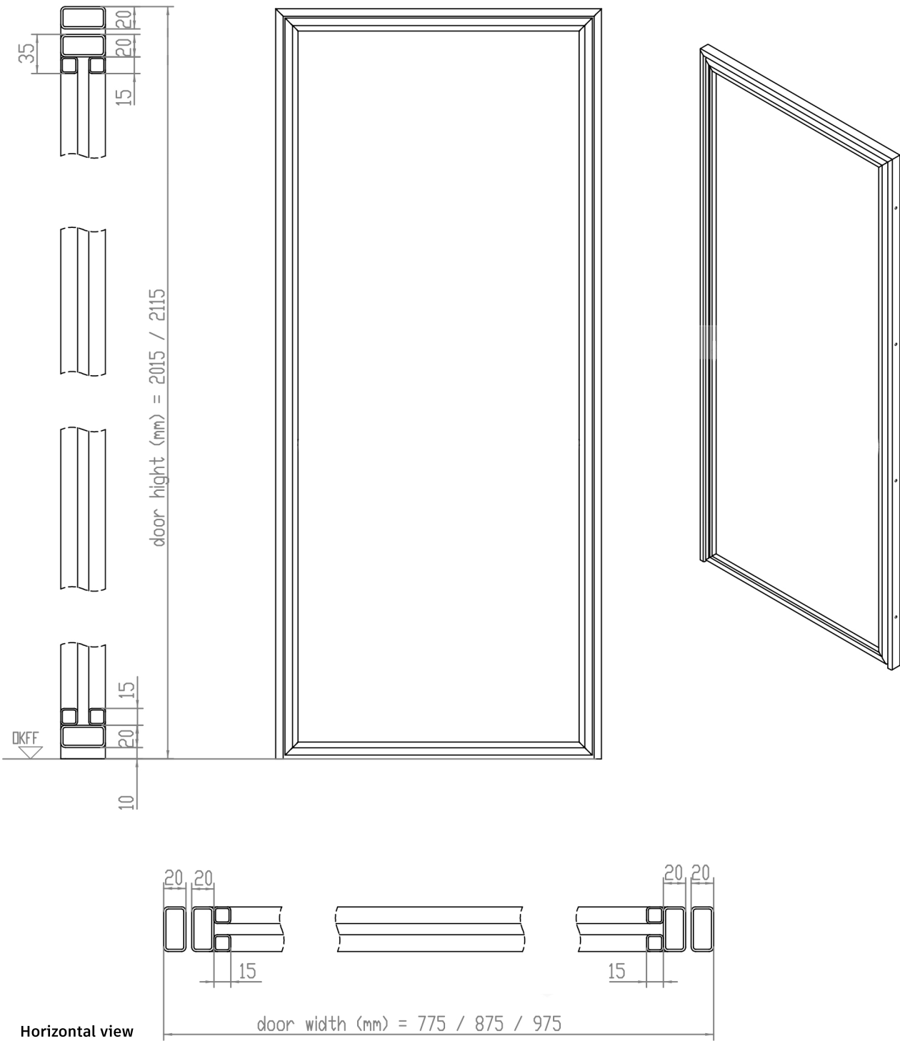
Single-leaf hinged door
